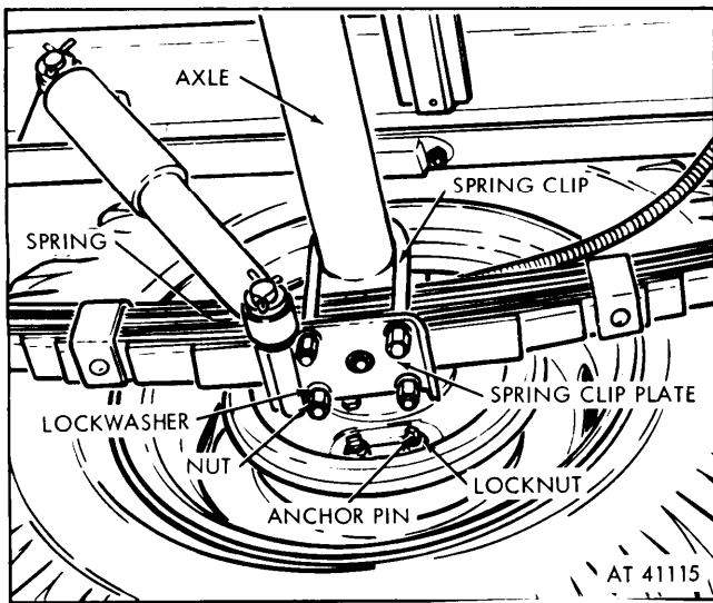
Figure 1-5. Axle installed.
