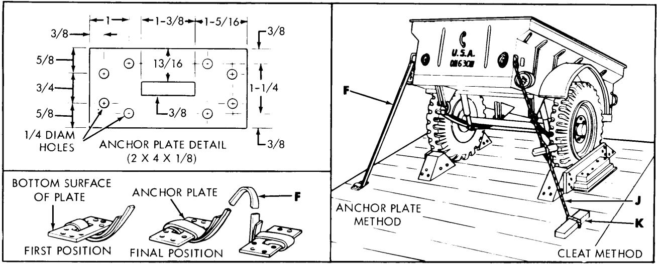
DETAIL A METHOD OF THREADING ANCHOR PLATE
