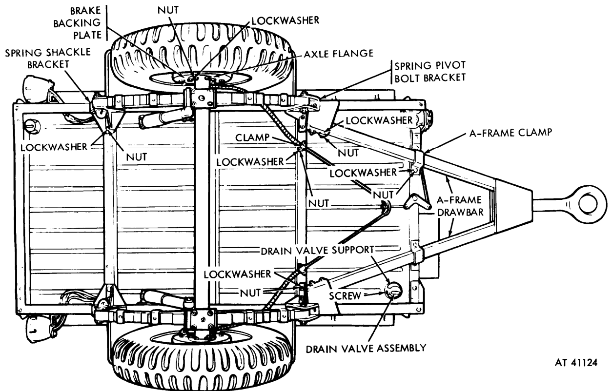
Figure 4-3. Trailer—bottom view.
