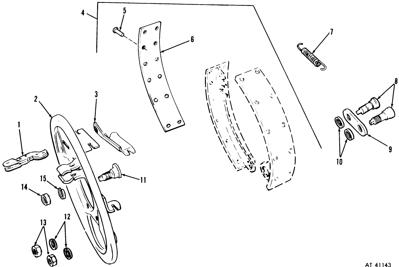
Figure C-8. Brake assembly.
