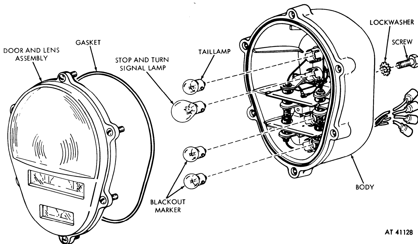
Figure 4-7. Lamp replacement.
