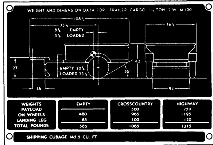
Figure 1-10. Name, Data, and service plates.
