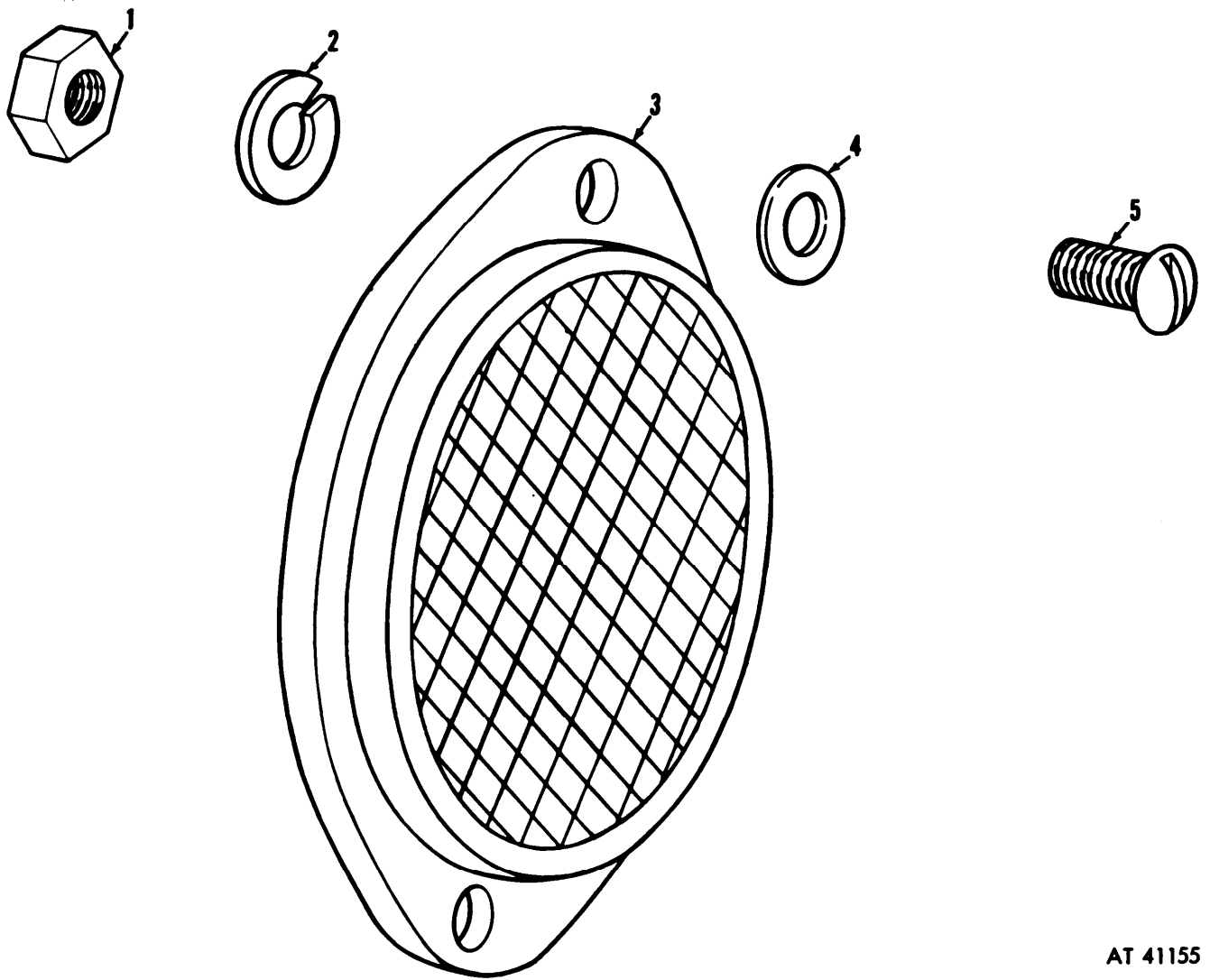
Figure C-20. Reflectors.
