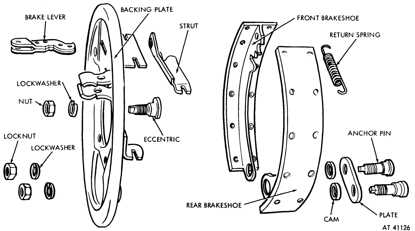
Figure 4-5. Brake assembly—exploded view.
