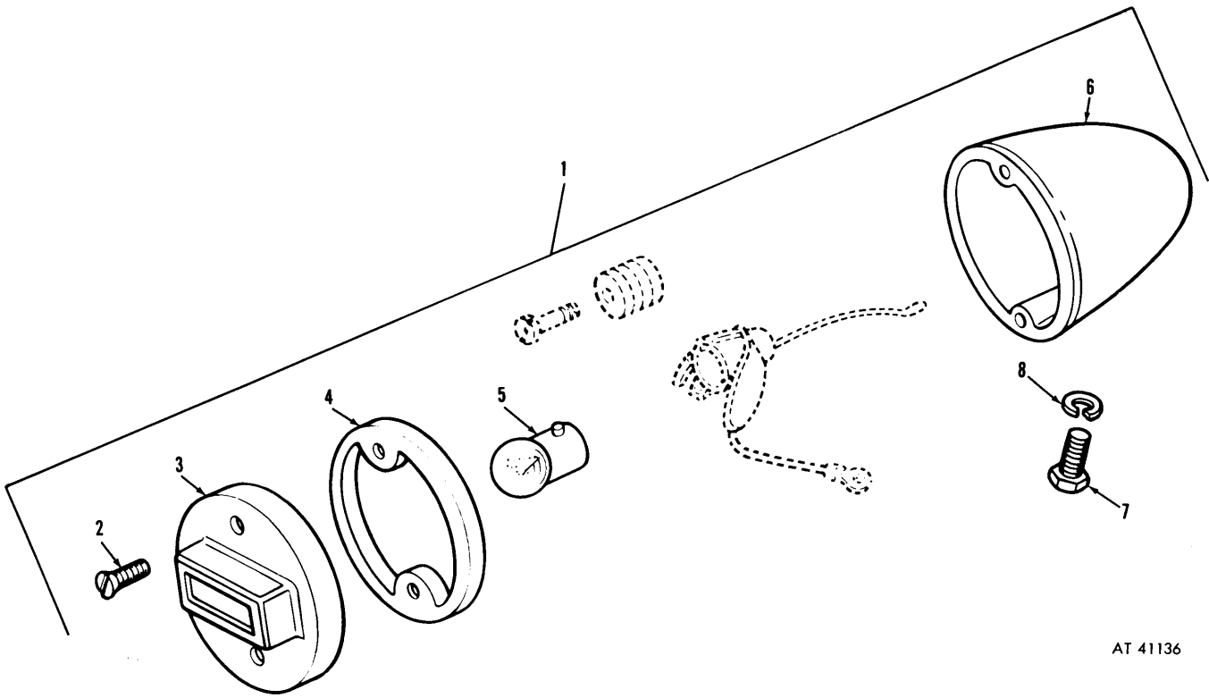
Figure C-1. Blackout-stoplight assembly.
