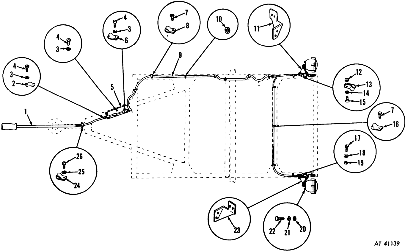
Figure C-4. Trailer wiring.
