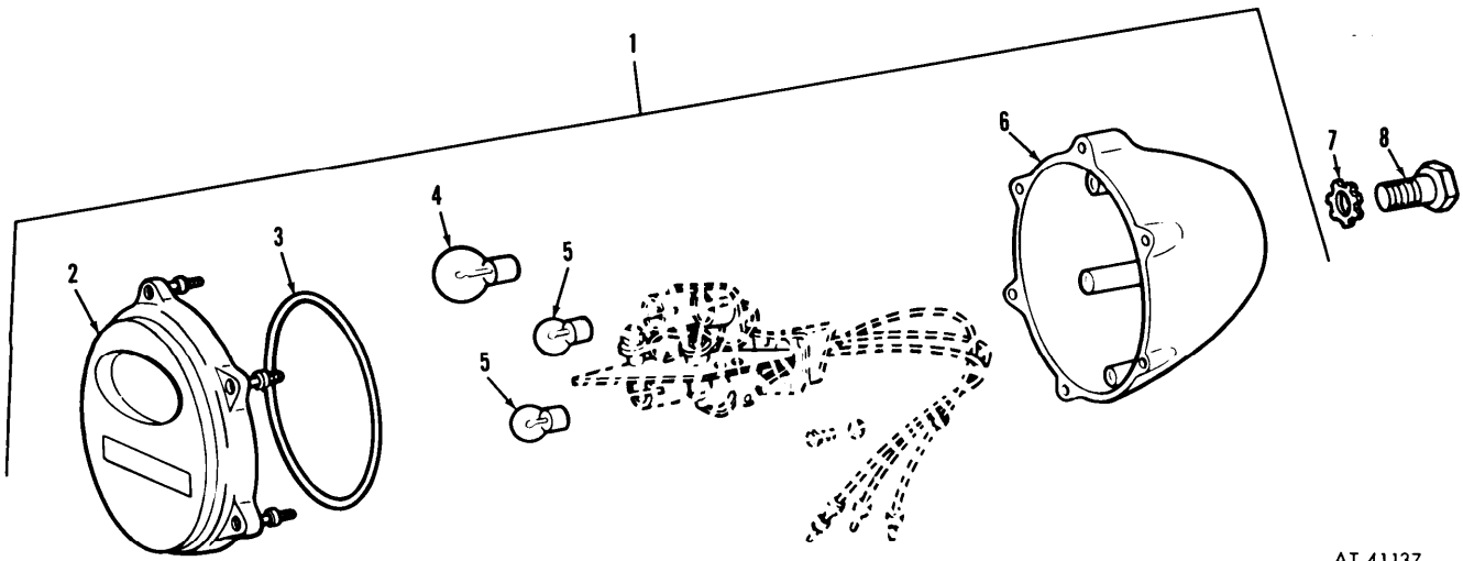
Figure C-1. Blackout-stoplight assembly.
