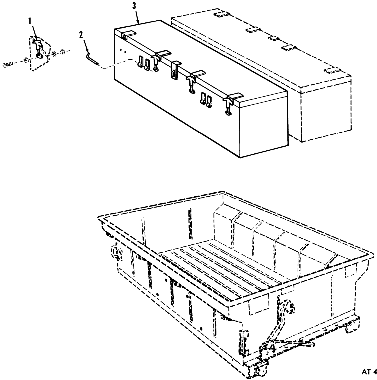
Figure C-17. Chest assembly (M367).
