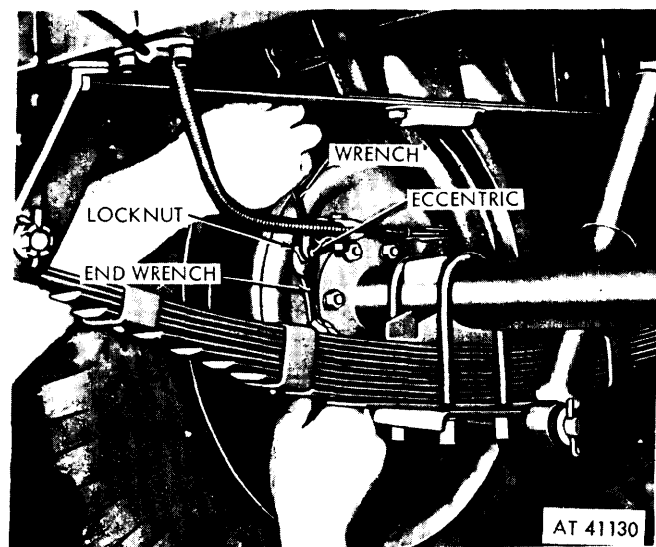
Figure 4-9. Brake adjustment with engineer's angle wrench.
